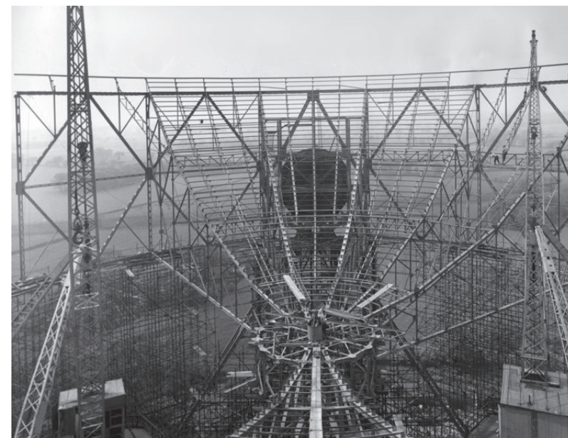
Jodrell Bank's Mark 1 radio telescope under construction.
