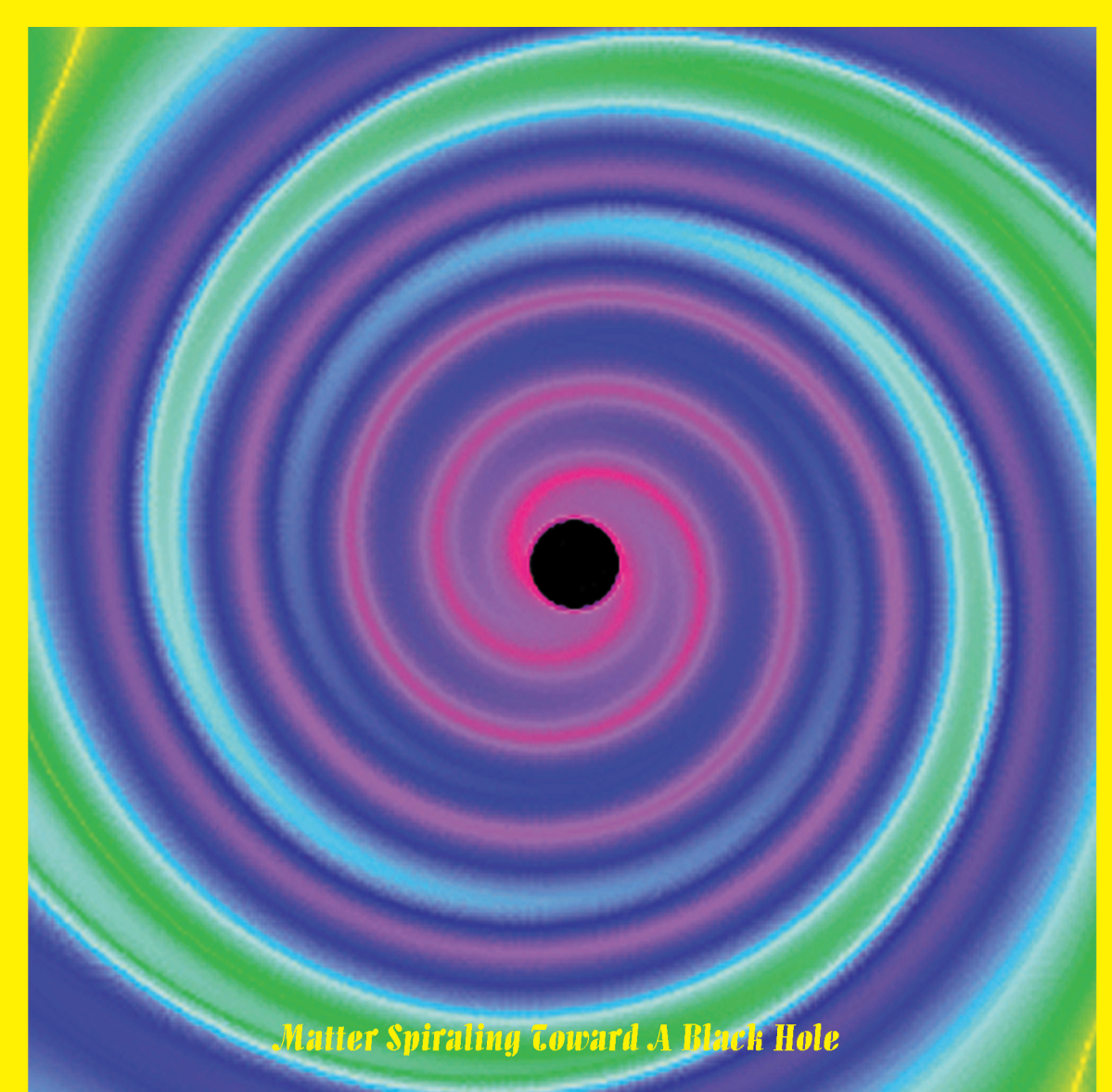
Active Galaxy
