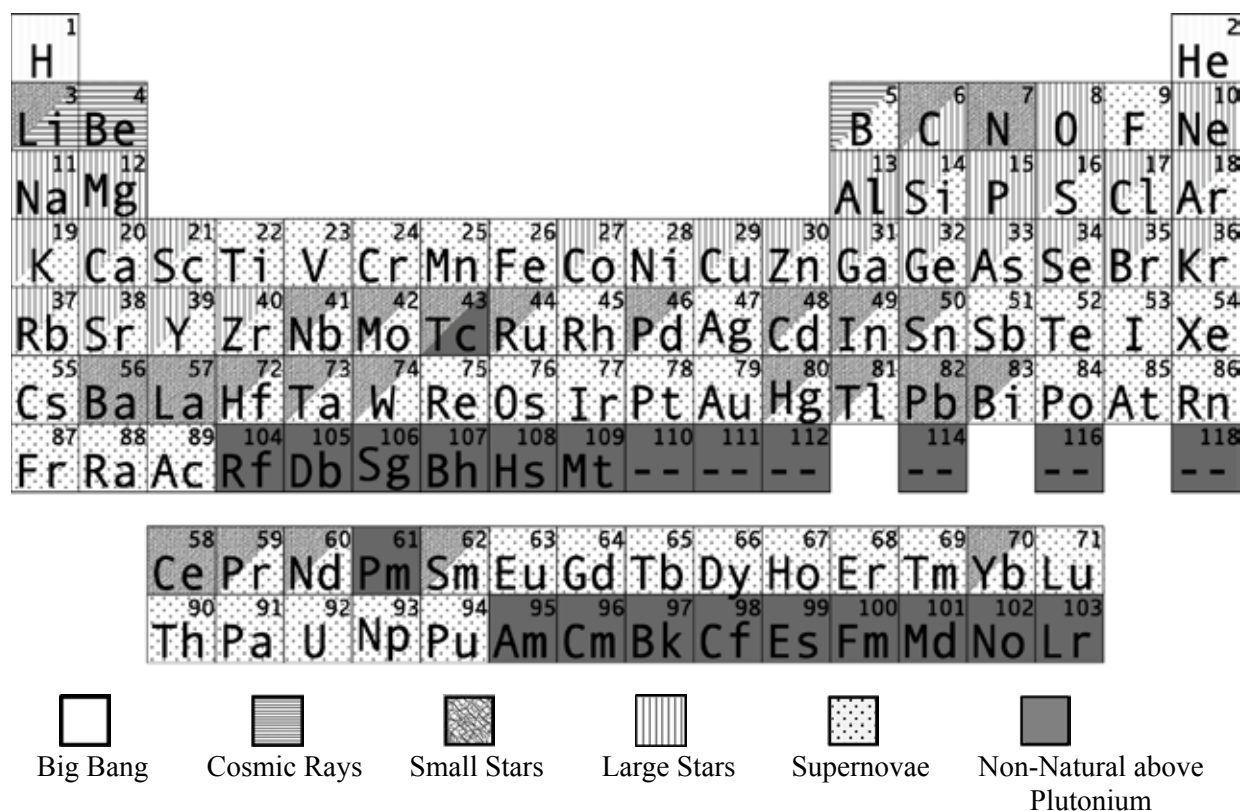
Figure 1: The Periodic Table of the Elements, coded according to the dominant processes which produce the elements.
