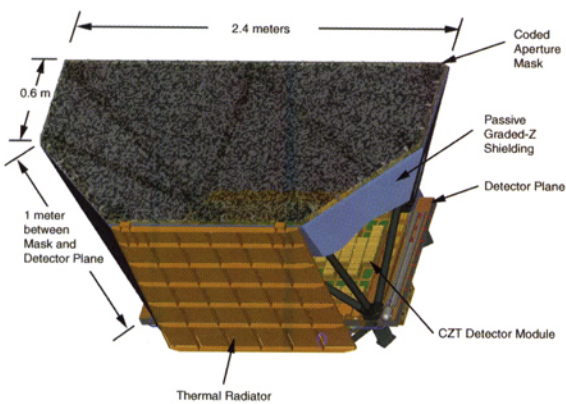
Swift BAT Instrument
