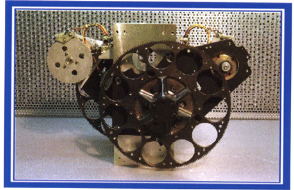
UVOT: UV/optical telescope filter wheel
